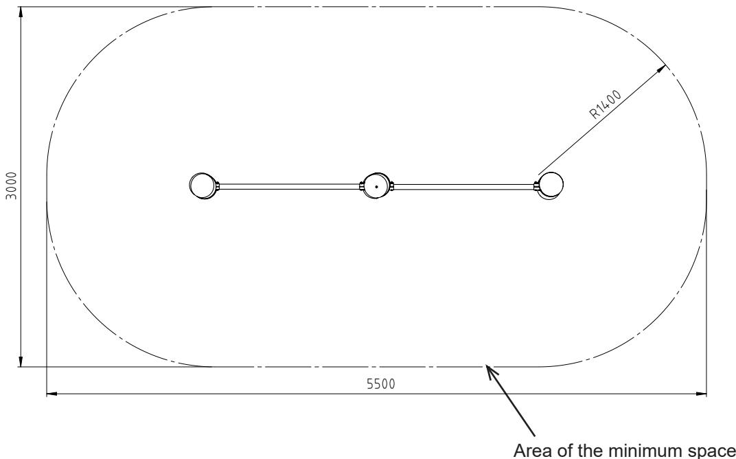
Diagram 4: Top view
